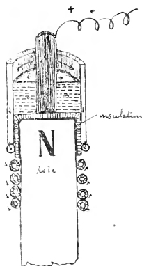
FIG. 50. Sectional diagram of electro-magnetic streaming. The small arrows show the direction of the electrical current and the large ones the movement of the mercury.
